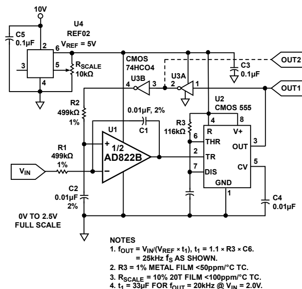
Figure 47. Single-Supply Voltage to Frequency Converter
