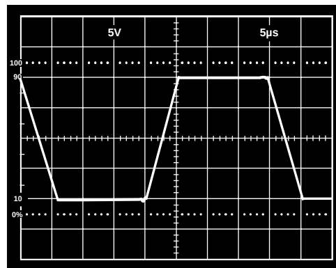
Figure 32. Large Signal Response Unity-Gain Follower; V_S = \pm 15 V, R_L = 10 \text{ k}\Omega
