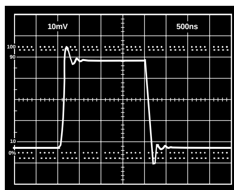
Figure 33. Small Signal Response Unity-Gain Follower; V_S = \pm 15 V, R_L = 10 \text{ k}\Omega
