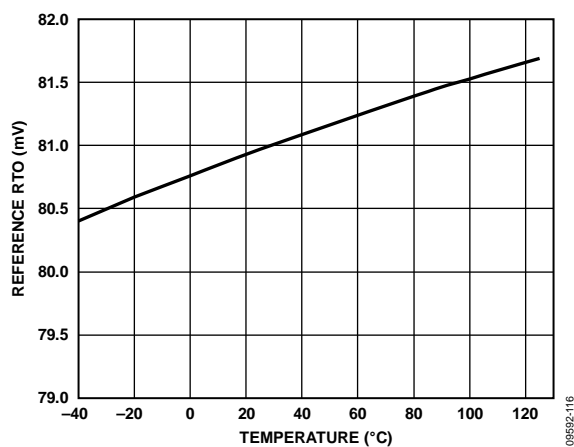
Figure 17. Internal Reference Voltage vs. Temperature (V_S = 5\text{ V}, V_S = NC, V_{CM} = 12\text{ V}, \text{Pin } 1 (+IN) \text{ and Pin } 8 (-IN) \text{ Shorted, Pin } 3 (ENB) \text{ Shorted to Pin } 4 (GND))
