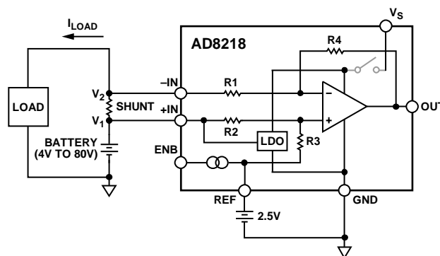
Figure 34. Bidirectional Operation Using a 2.5 V Reference Input
