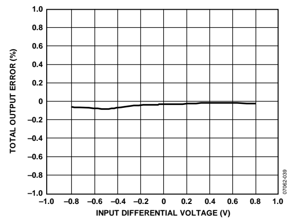
Figure 18. Output Error (%) vs. Differential Input Voltage (Bidirectional Operation ( V_{\text{REF}1} and V_{\text{REF}2} Connected to 2.5 V))
