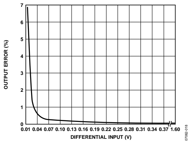
Figure 17. Output Error (%) vs. Differential Input Voltage (Unidirectional Operation ( V_{\text{REF}1} and V_{\text{REF}2} Connected to GND))
