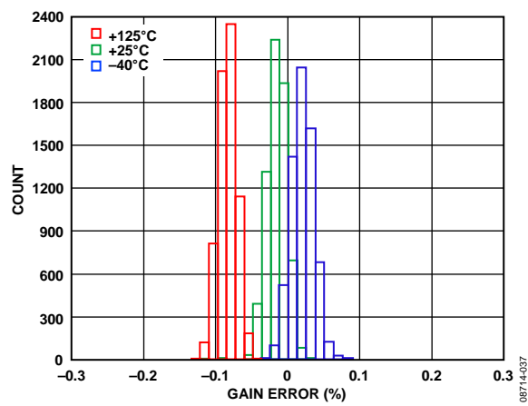
Figure 23. Gain Error
