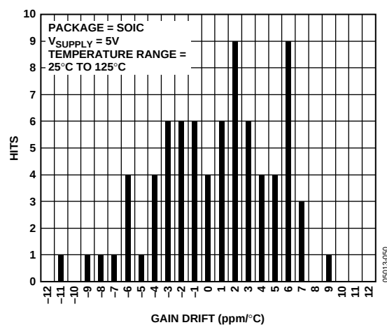
Figure 39. Gain Drift Distribution, SOIC, Temperature Range = 25°C to 125°C
