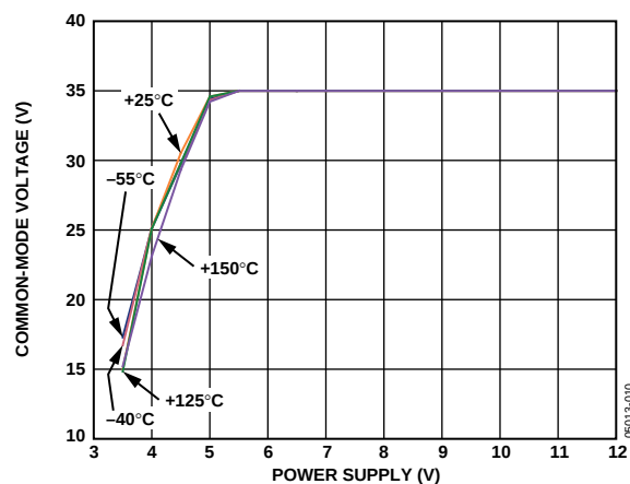
Figure 10. Positive Common-Mode Voltage vs. Voltage Supply
