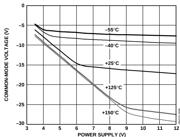
Figure 9. Negative Common-Mode Voltage vs. Voltage Supply
