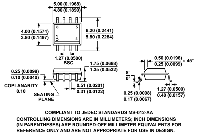
Figure 53. 8-Lead Standard Small Outline Package [SOIC_N] Narrow Body (R-8)
