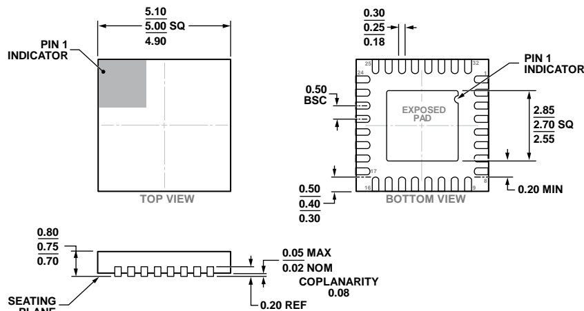
Figure 27. 32-Lead Lead Frame Chip Scale Package [LFCSP] 5 mm × 5 mm Body and 0.75 mm Package Height (CP-32-21)
