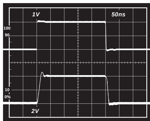
TPC 29. Noninverting Large Signal Pulse Response; V_S = \pm 5\text{ V} , C_F = 1\text{ pF} , R_L = 1\text{ kW}
