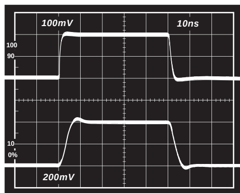
TPC 30. Noninverting Small Signal Pulse Response; V_S = \pm 5\text{ V} , C_F = 1\text{ pF} , R_L = 150\text{ W}
