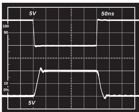
TPC 25. Inverter Large Signal Pulse Response; V_S = \pm 15\text{ V} , C_F = 1\text{ pF} , R_L = 1\text{ kW}
