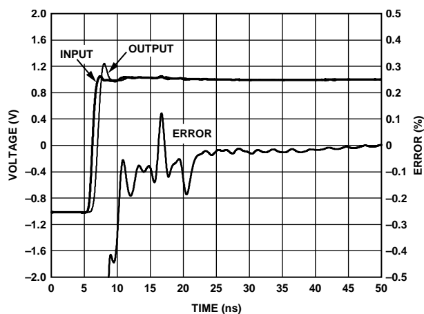
Figure 22. Settling Time
