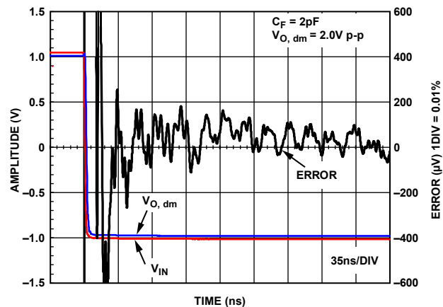
Figure 36. Settling Time (0.01%)
