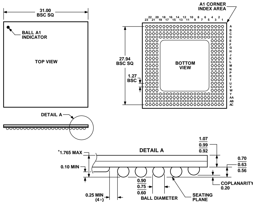
Figure 73. 304-Ball Ball Grid Array, Thermally Enhanced [BGA_ED] (BP-304) Dimensions shown in millimeters
