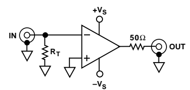
Inverting Configuration
