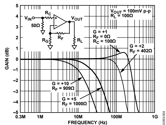
Figure 4. Frequency Response
