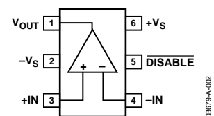
Figure 2. SC70-6 (KS)
