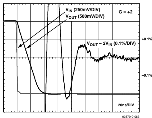
Figure 34. 0.1% Short-Term Settling Time
