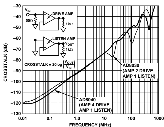
Figure 36. AD8030/AD8040 Crosstalk vs. Frequency
