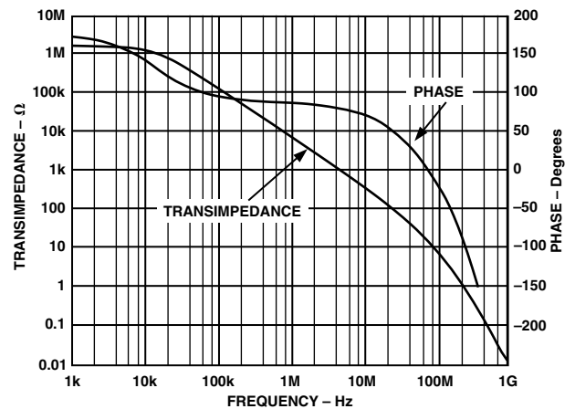
TPC 23. Open Loop Transimpedance and Phase
