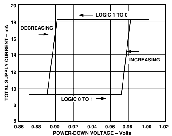
TPC 24. Power-Up/Down Threshold Voltage
