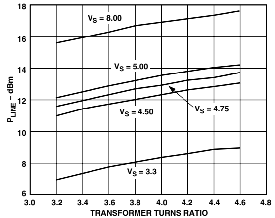
TPC 22. Line Power vs. Turns Ratio; -75 dBc Out-of-Band SFDR, f = 361 kHz
