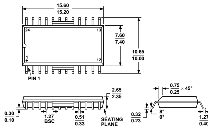
Figure 50. 24-Lead Batwing SOIC, Thermally Enhanced w/Fused Leads [SOIC_W_BAT] (RB-24) Dimensions shown in millimeters
