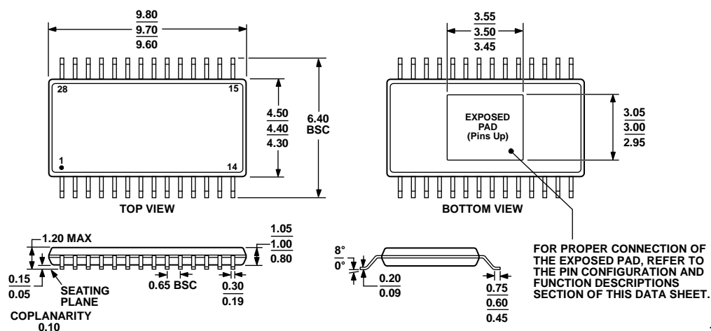
Figure 51. 28-Lead Thin Shrink Small Outline With Exposed Pad [TSSOP_EP] (RE-28-1) Dimensions shown in millimeters
