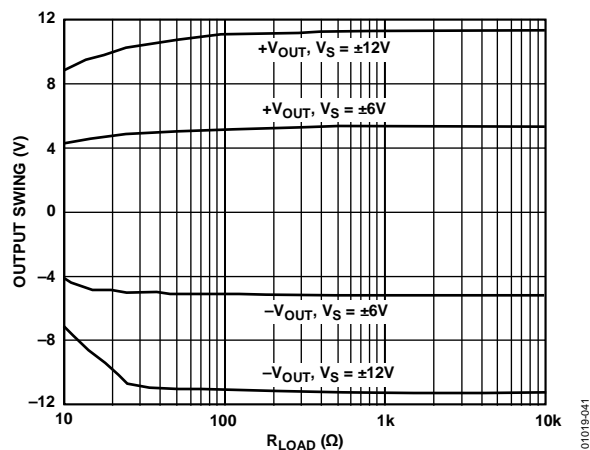
Figure 39. Output Voltage vs. R_{LOAD}
