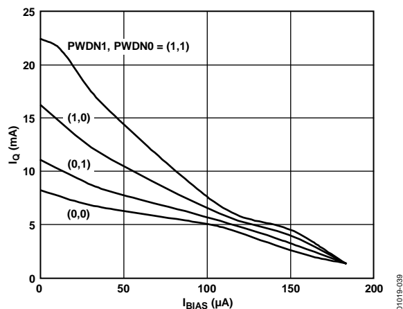
Figure 37. I_Q vs. I_{BIAS} Current; V_S = \pm 12V
