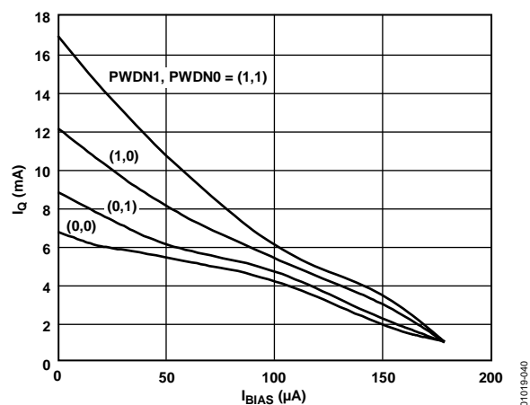
Figure 38. I_Q vs. I_{BIAS} Current; V_S = \pm 6V
