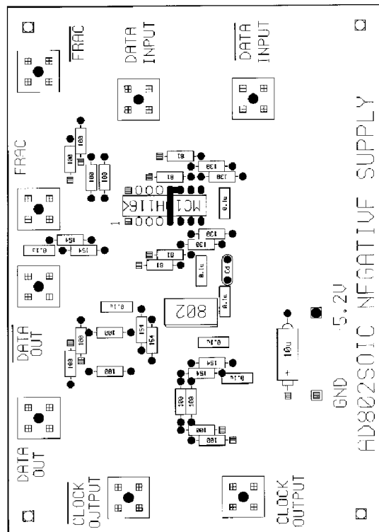
Figure 28. Negative Supply Configuration: Solder Side
