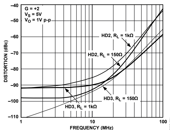
Figure 21. AD8007 Second and Third Harmonic Distortion vs. Frequency and R_L
