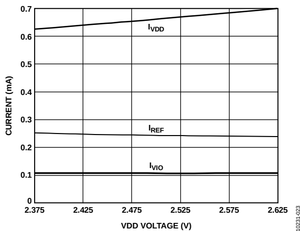
Figure 21. Operating Currents vs. Supply (AD7988-5)
