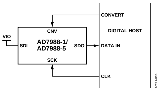
Figure 33. 3-Wire \overline{\text{CS}} Mode Connection Diagram
