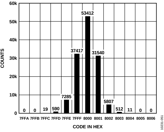
Figure 16. Histogram of a DC Input at the Code Center, V_{REF} = 2.5\text{ V}
