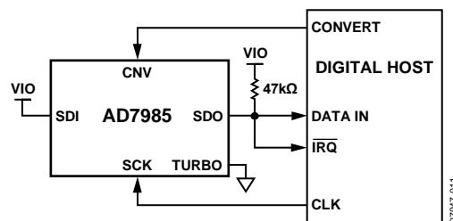
Figure 28. \overline{CS} Mode, 3-Wire with Busy Indicator Connection Diagram ( \overline{SDI} High)
