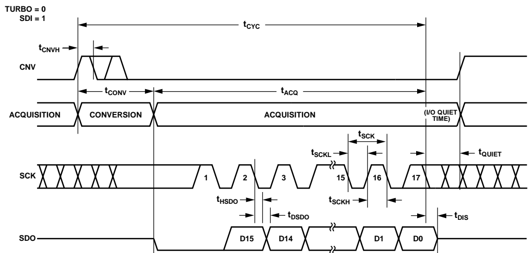
Figure 29. \overline{CS} Mode, 3-Wire with Busy Indicator Serial Interface Timing ( \overline{SDI} High)
