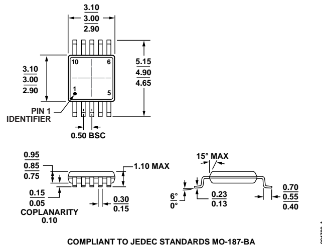
Figure 56. 10-Lead Mini Small Outline Package [MSOP] (RM-10)
