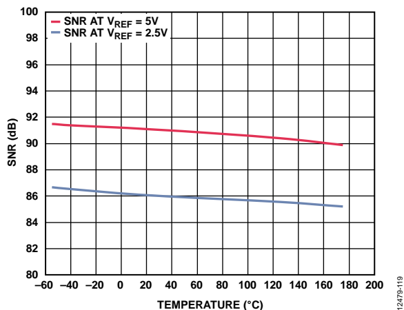
Figure 24. SNR vs. Temperature, MSOP
