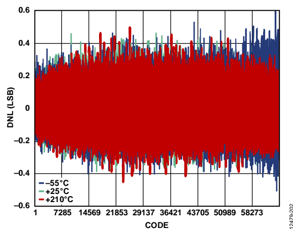
Figure 14. Differential Nonlinearity (DNL) vs. Code and Temperature, V_{REF} = 2.5\text{ V} , FLATPACK
