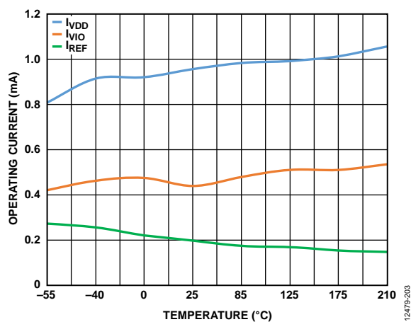
Figure 33. Operating Current vs. Temperature, FLATPACK
