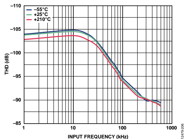
Figure 28. THD vs. Input Frequency, FLATPACK
