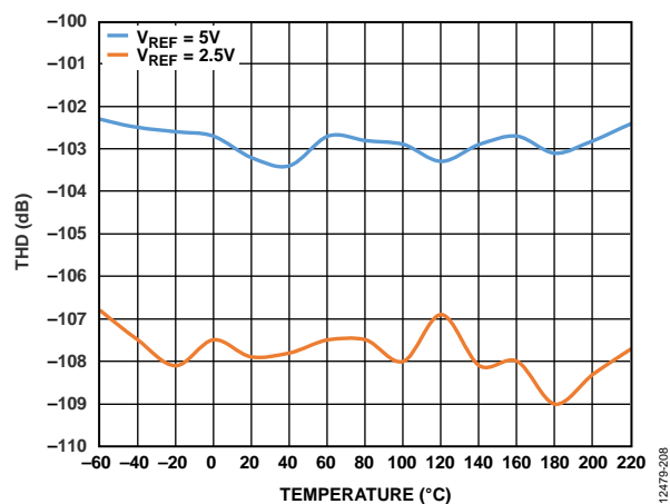
Figure 32. THD vs. Temperature, FLATPACK
