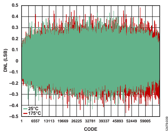
Figure 11. Differential Nonlinearity (DNL) vs. Code and Temperature, V_{REF} = 2.5\text{ V} , MSOP
