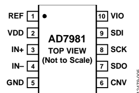
Figure 4. 10-Lead FLATPACK Pin Configuration
