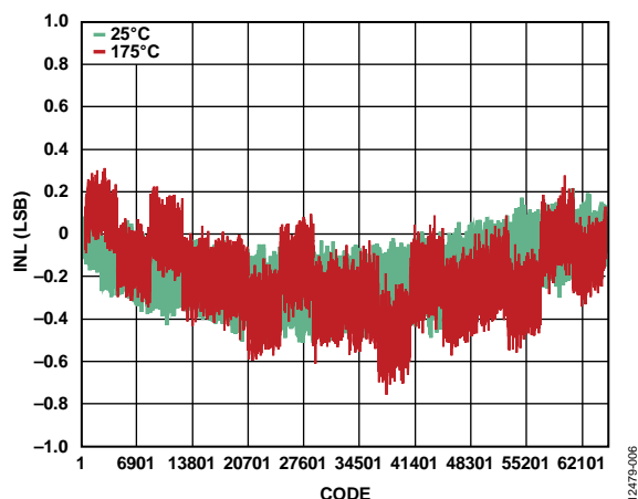
Figure 5. Integral Nonlinearity (INL) vs. Code and Temperature, V_{REF} = 5.0\text{ V} , MSOP
