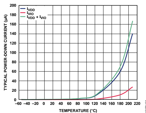
Figure 34. Typical Power-Down Current vs. Temperature
