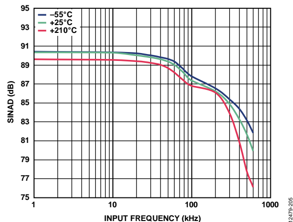
Figure 26. SINAD vs. Input Frequency, FLATPACK
