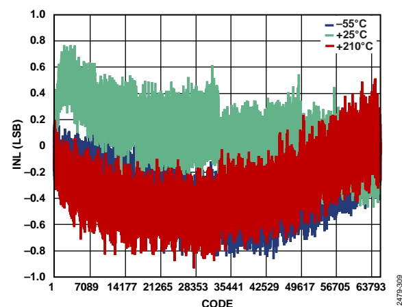
Figure 9. Integral Nonlinearity (INL) vs. Code and Temperature, V_{REF} = 2.5\text{ V} , FLATPACK
