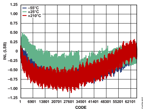
Figure 8. Integral Nonlinearity (INL) vs. Code and Temperature, V_{REF} = 5.0\text{ V} , FLATPACK
