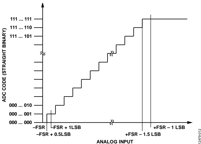
Figure 36. ADC Ideal Transfer Function
