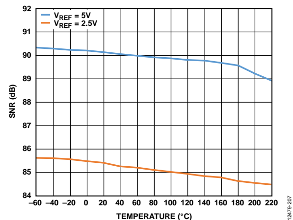
Figure 27. SNR vs. Temperature, FLATPACK
