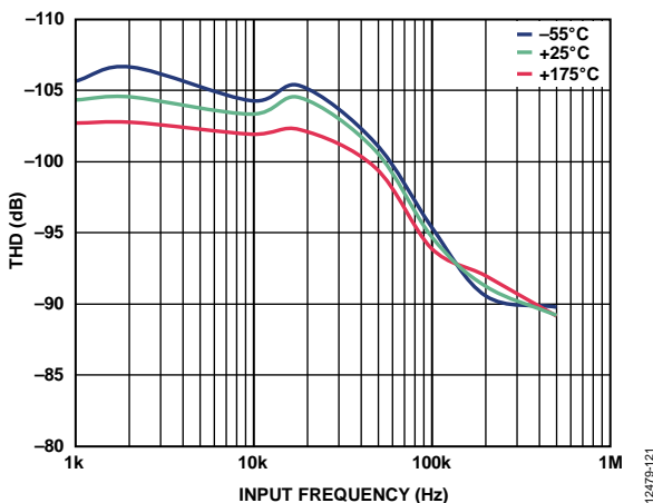
Figure 25. THD vs. Frequency, MSOP
