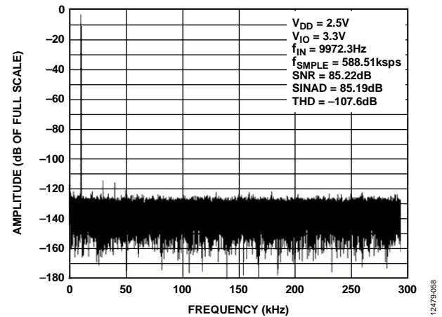
Figure 20. 10 kHz FFT, V_{REF} = 2.5\text{ V}
