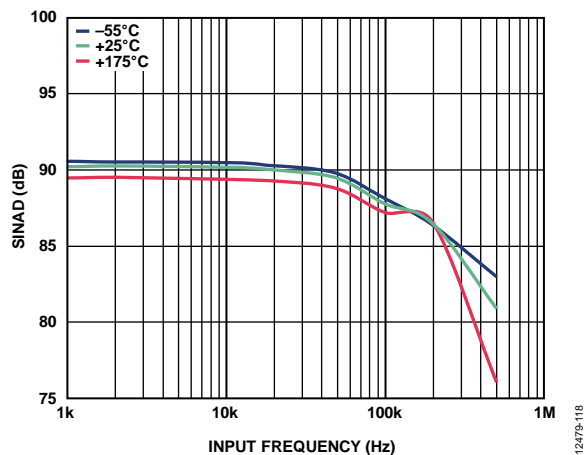
Figure 23. SINAD vs. Input Frequency, MSOP
