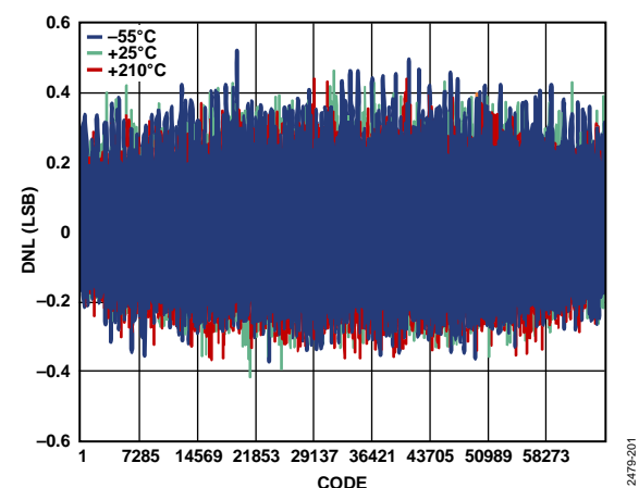
Figure 10. Differential Nonlinearity (DNL) vs. Code and Temperature, V_{REF} = 5.0\text{ V} , FLATPACK
