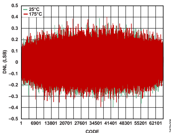
Figure 7. Differential Nonlinearity (DNL) vs. Code and Temperature, V_{REF} = 5.0\text{ V} , MSOP
