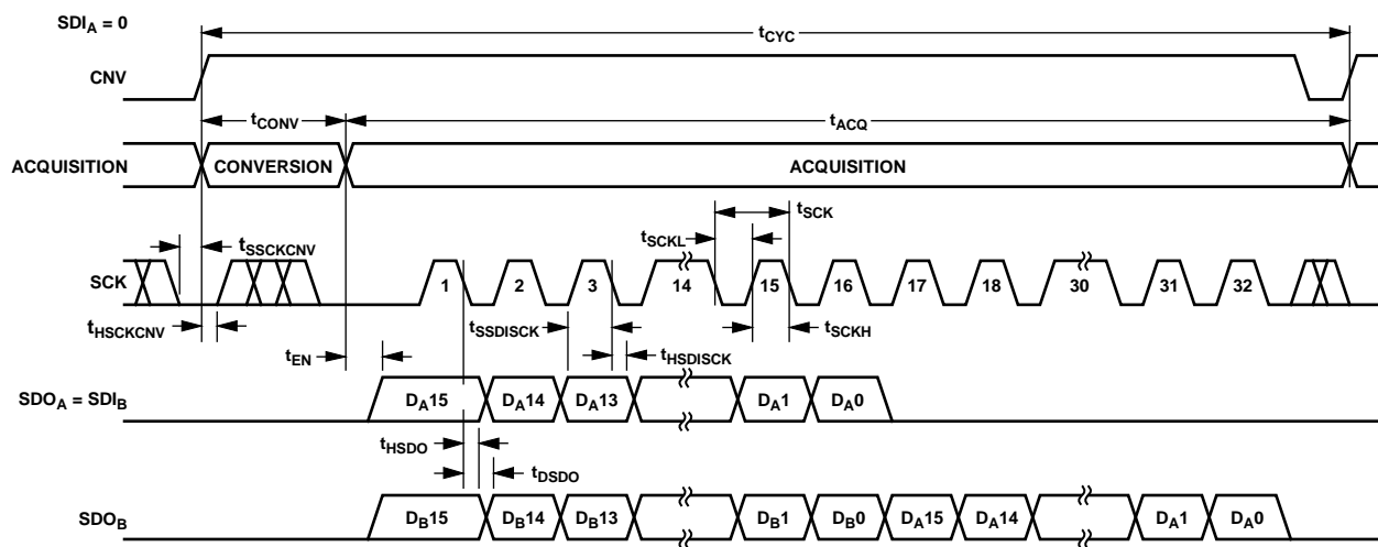
Figure 50. Chain Mode Without Busy Indicator Serial Interface Timing
