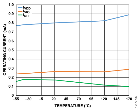
Figure 30. Operating Current vs. Temperature, MSOP
