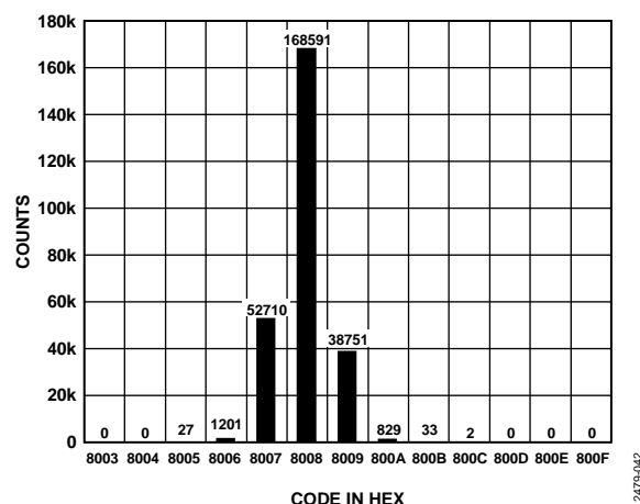
Figure 13. Histogram of a DC Input at the Code Center, V_{REF} = 5.0\text{ V}
