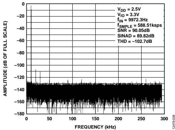
Figure 17. 10 kHz FFT, V_{REF} = 5.0\text{ V}
