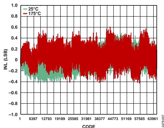
Figure 6. Integral Nonlinearity (INL) vs. Code and Temperature, V_{REF} = 2.5\text{ V} , MSOP
