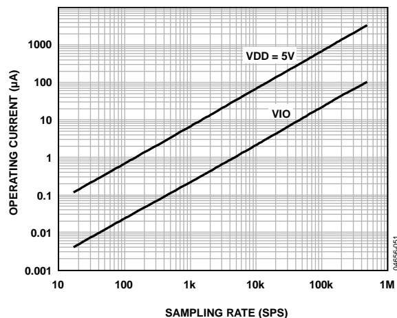
Figure 30. Operating Currents vs. Sampling Rate
