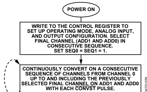
Figure 31. Consecutive Sequence Mode Flow Chart
