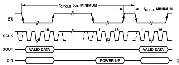
Figure 28. General Timing Diagram
