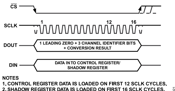
Figure 21. Normal Mode Operation
