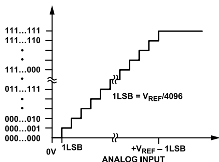
Figure 17. Straight Binary Transfer Characteristic
