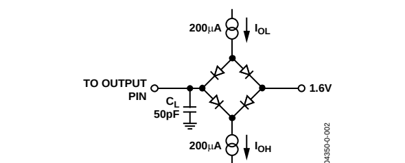
Figure 2. Load Circuit for Digital Output Timing Specifications
