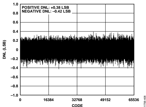
Figure 8. Differential Nonlinearity vs. Code, V_{REF} = 5\text{ V}
