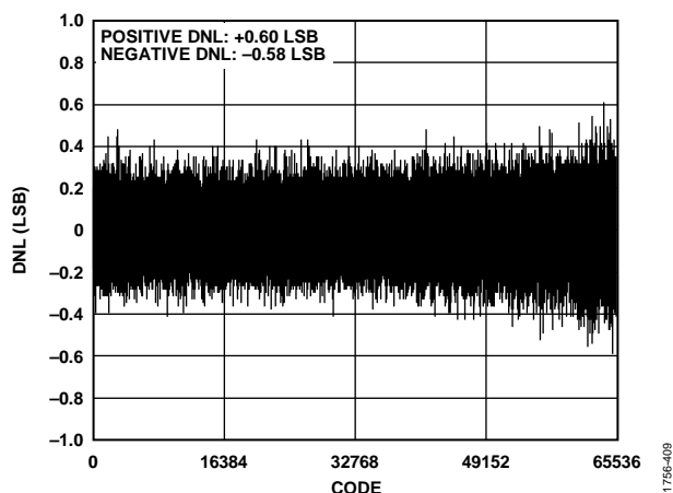
Figure 9. Differential Nonlinearity vs. Code, V_{REF} = 2.5\text{ V}
