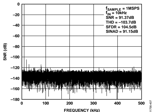
Figure 7. FFT Plot, V_{REF} = 5\text{ V}
