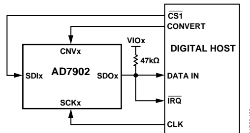
Figure 44. \overline{\text{CS}} Mode, 4-Wire Interface with a Busy Indicator Connection Diagram
