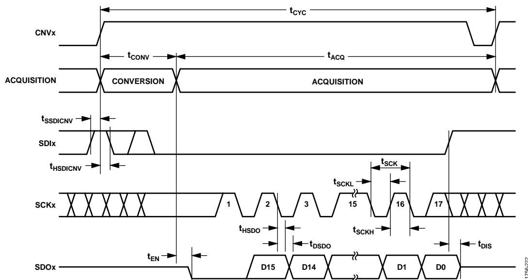
Figure 45. \overline{\text{CS}} Mode, 4-Wire Interface with a Busy Indicator Serial Interface Timing
