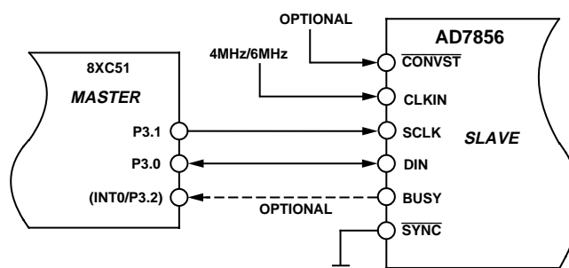
Figure 37. 8XC51/PIC16C42 Interface
