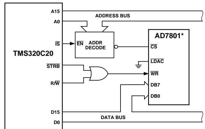
Figure 30. AD7801-TMS320C20 Interface
