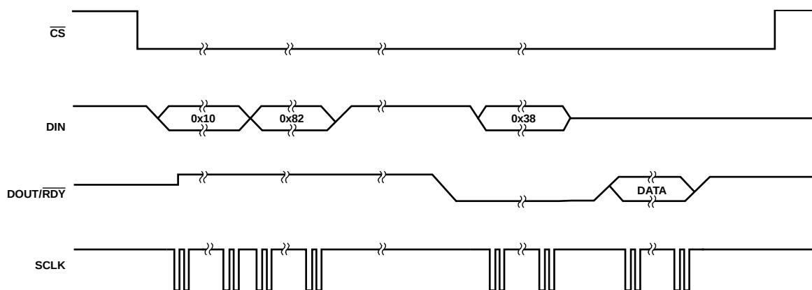
Figure 13. Single Conversion
