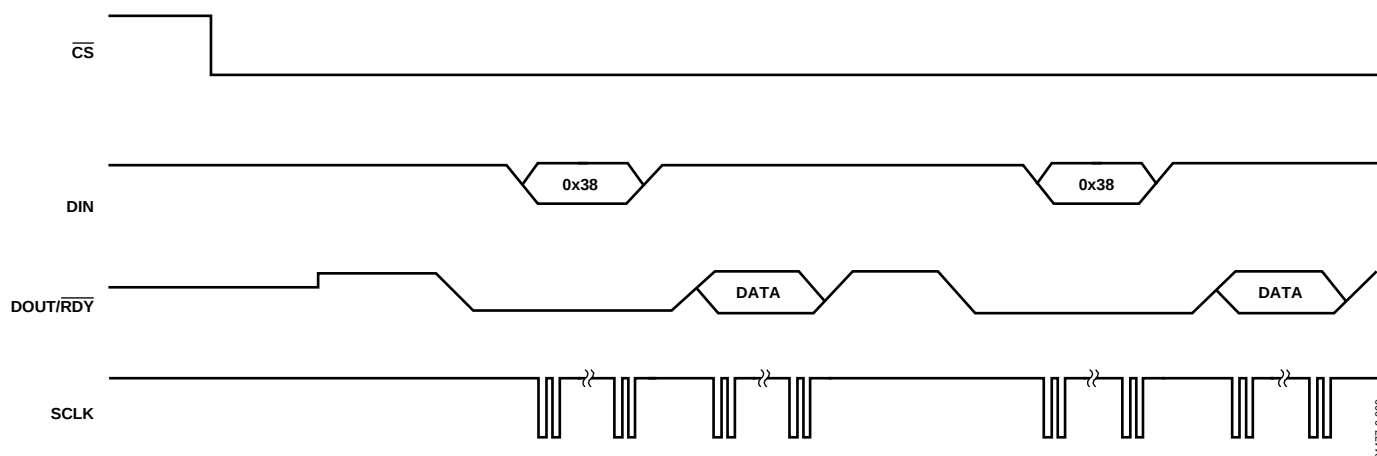
Figure 14. Continuous Conversion
