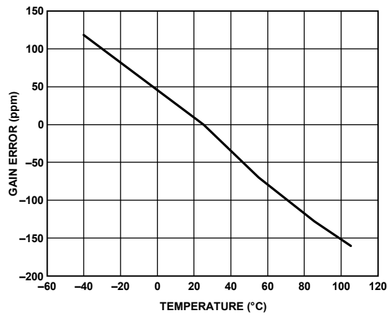
Figure 19. Gain Error vs. Temperature (Gain = 128)
