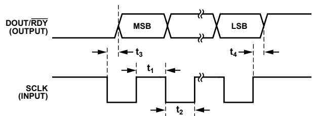
Figure 3. Read Cycle Timing Diagram
