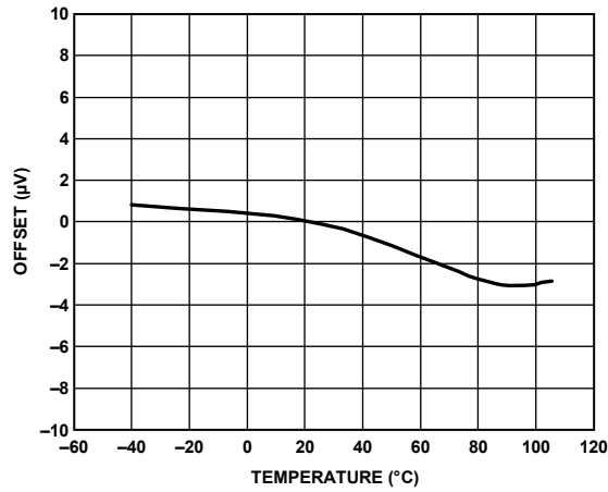
Figure 18. Offset vs. Temperature (Gain = 128)
