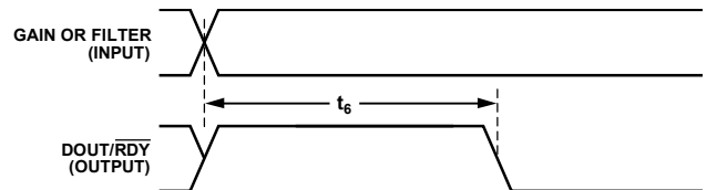
Figure 5. Changing Gain or Filter Option
