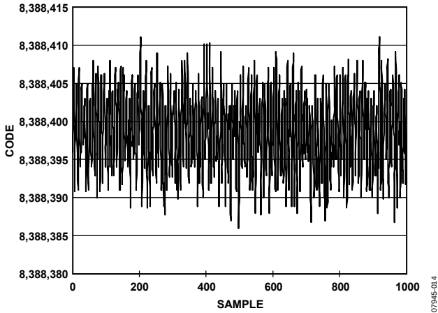
Figure 14. Noise ( V_{REF} = AV_{DD} , Update Rate = 10 Hz, Gain = 1)
