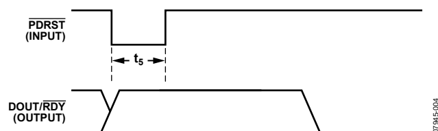
Figure 4. Resetting the AD7780
