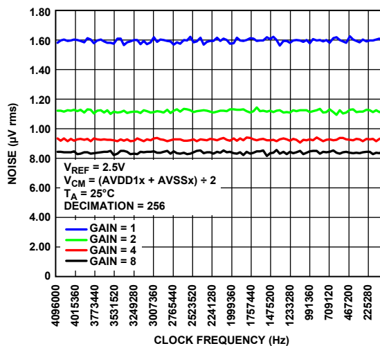
Figure 29. Noise vs. Clock Frequency, Low Power Mode
