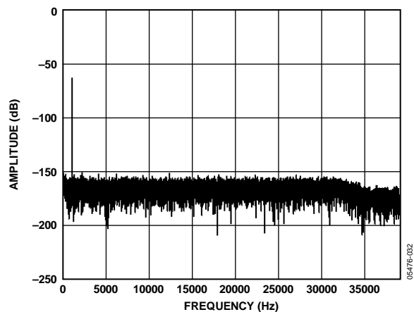
Figure 8. Normal Mode FFT, 1 kHz, -60 dB Input Tone, 256x Decimation
