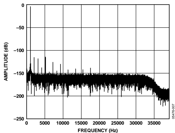
Figure 6. Normal Mode FFT, 1 kHz, -0.5 dB Input Tone, 256x Decimation
