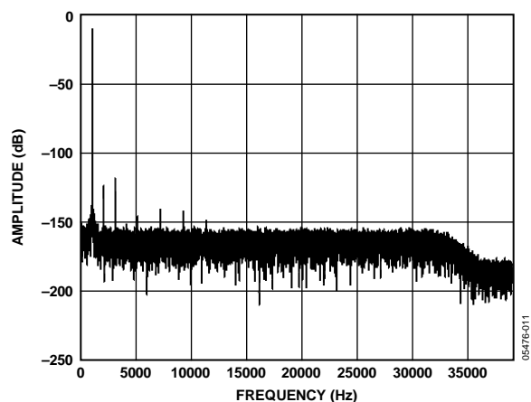
Figure 7. Normal Mode FFT, 1 kHz, -0.6 dB Input Tone, 256x Decimation
