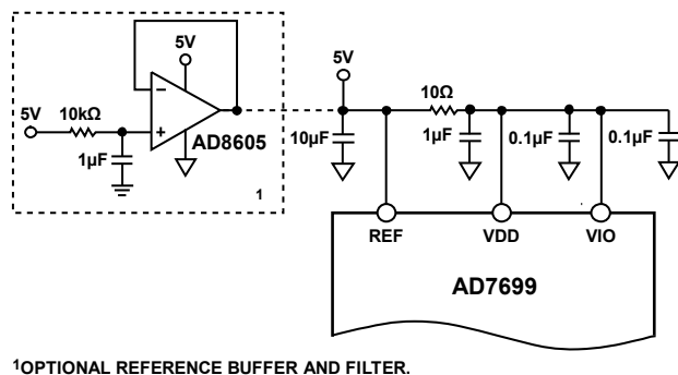
Figure 36. Example of an Application Circuit
