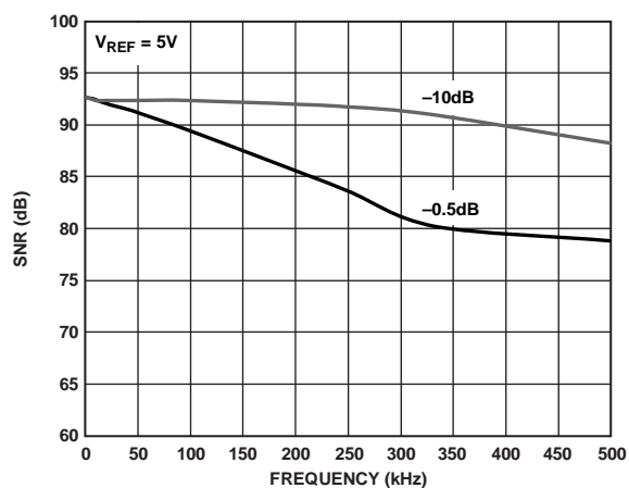
Figure 12. SNR vs. Frequency
