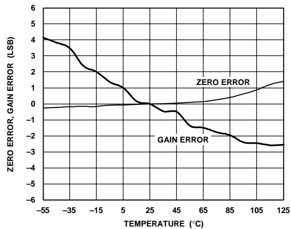
Figure 19. Zero Error and Gain Error vs. Temperature
