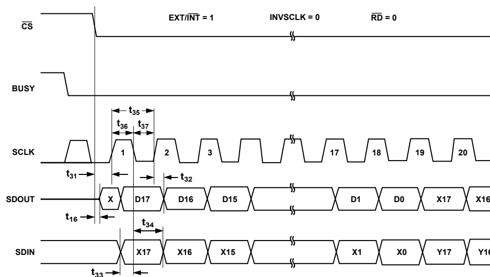
Figure 41. Slave Serial Data Timing for Reading (Read after Convert)
