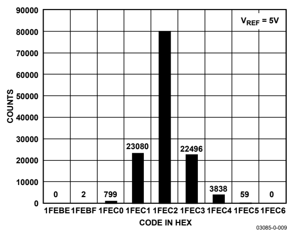
Figure 10. Histogram of 131,072 Conversions of a DC Input at the Code Center
