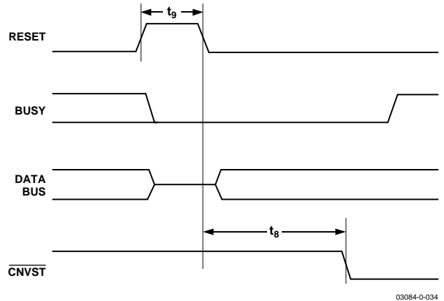
Figure 28. RESET Timing
