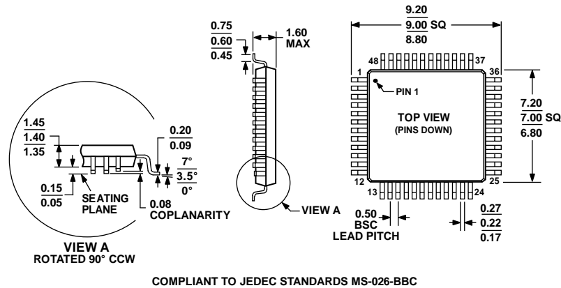
Figure 39. 48-Lead Low Profile Quad Flat Package [LQFP] (ST-48) Dimensions shown in millimeters
