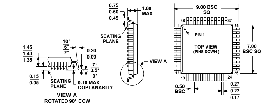
Figure 47. 48-Lead Low Profile Quad Flat Package [LQFP] (ST-48)
