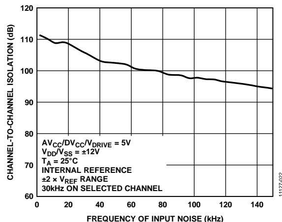
Figure 18. Channel-to-Channel Isolation
