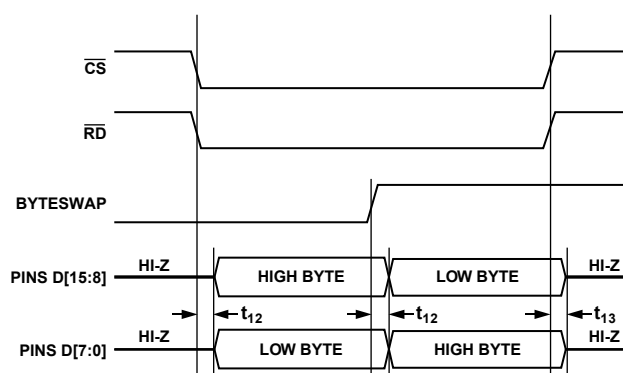
Figure 31. 8-Bit Parallel Interface
