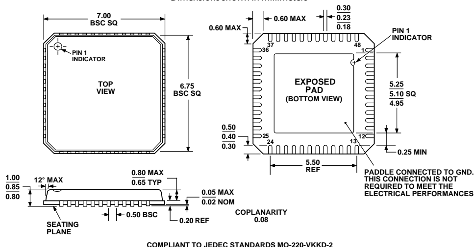
Figure 44. 48-Lead Lead Frame Chip Scale Package [LFCSP_VQ] 7 mm x 7 mm Body, Very Thin Quad (CP-48-1)
