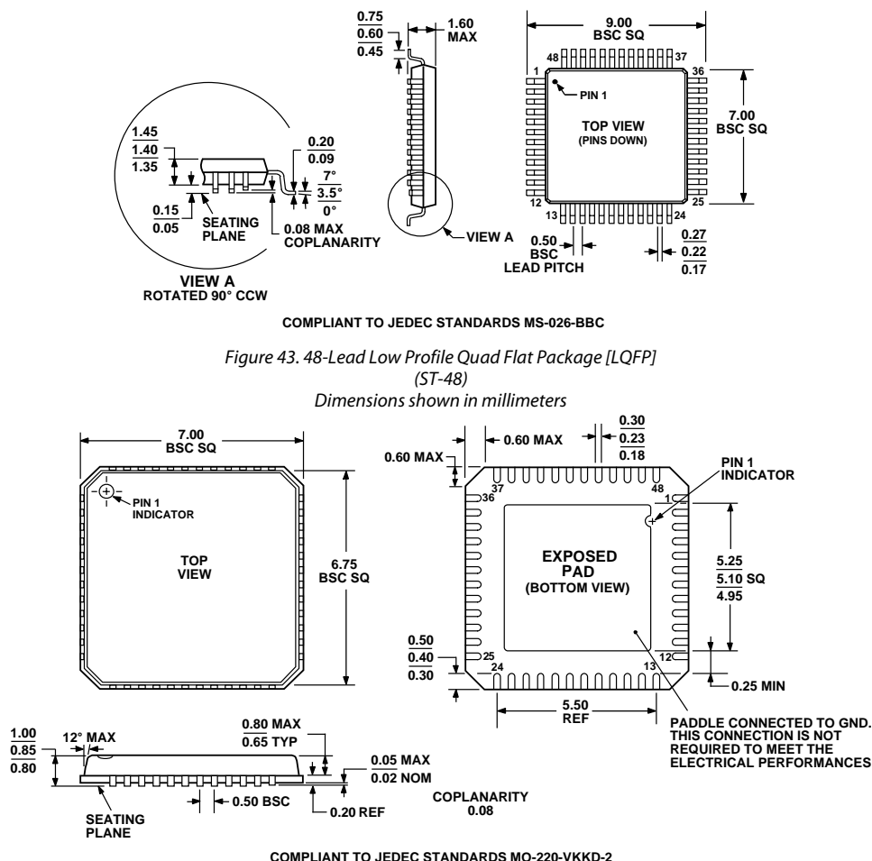
Figure 44. 48-Lead Lead Frame Chip Scale Package [LFCSP_VQ] 7 mm x 7 mm Body, Very Thin Quad (CP-48-1)
