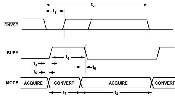
Figure 32. Basic Conversion Timing
