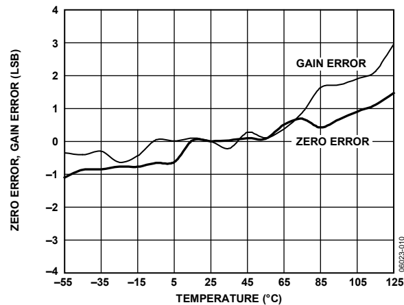
Figure 12. Zero Error, Gain Error vs. Temperature
