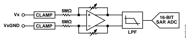
Figure 42. Analog Input Circuitry for Each Channel
