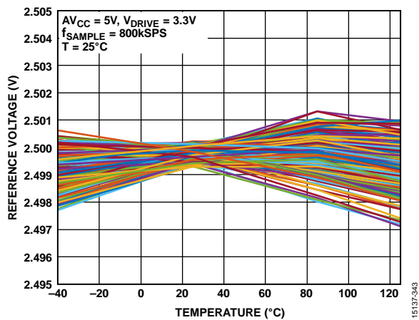
Figure 22. Reference Drift
