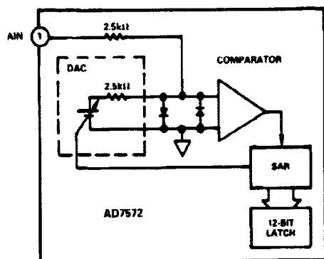
Figure 4. AD7572 AIN Input
