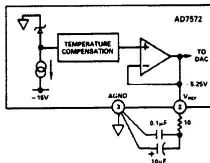
Figure 7. AD7572 Internal -5.25V Reference
