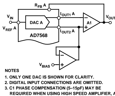
Figure 17. Single Supply Current-Mode Operation
