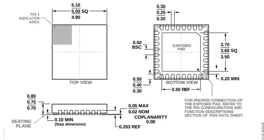
Figure 35. 32-Lead Lead Frame Chip Scale Package [LFCSP_SS] 5 mm x 5 mm Body with Side Solderable Leads (CS-32-3) Dimensions shown in millimeters
