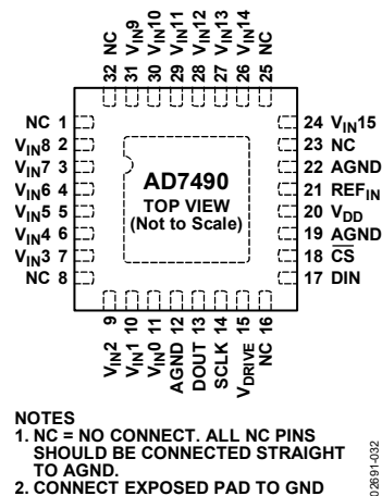
Figure 4. 32-Lead LFCSP Pin Configuration
