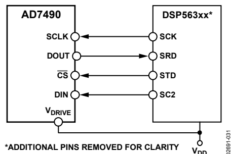
Figure 32. Interfacing to the DSP563xx
