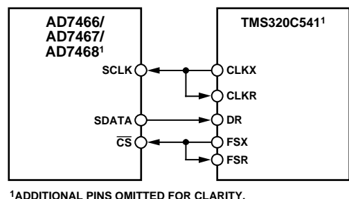
Figure 32. Interfacing to the TMS320C541
