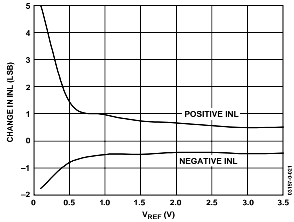
Figure 12. Change in INL vs. V_{REF} for V_{DD} = 5\text{ V}
