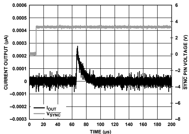
Figure 18. Current Output (I OUT ) and \overline{\text{SYNC}} Pin Voltage (V SYNC ) vs. Time on Output Enable
