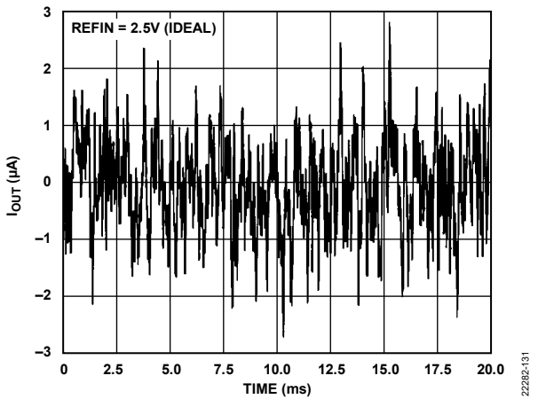
Figure 24. Peak-to-Peak Noise (100 kHz Bandwidth)
