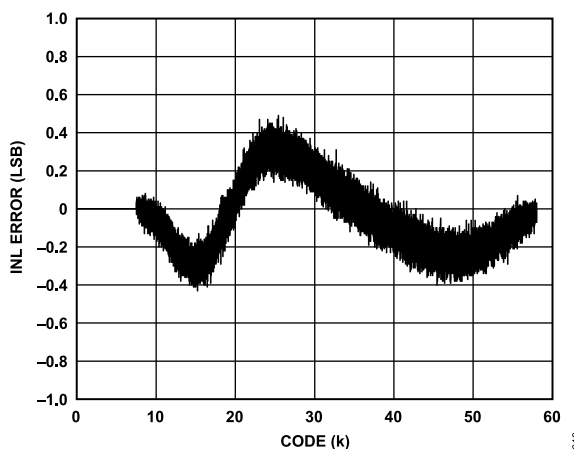
Figure 10. Typical INL Error
