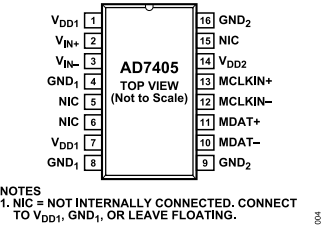
Figure 4. Pin Configuration
