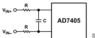
Figure 28. Differential RC Filter Input Network
